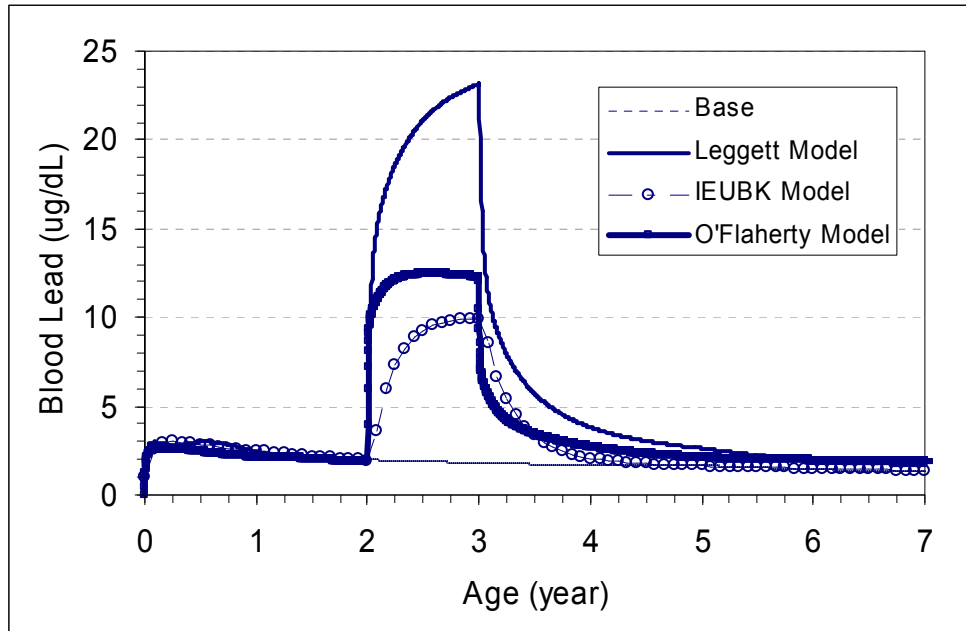
Figure 3-13. Blood Lead Concentrations in Children Predicted by the O'Flaherty, IEUBK, and Leggett Models*
